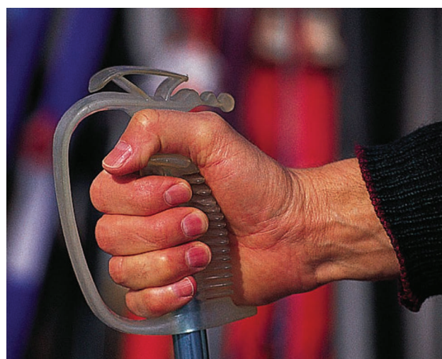
Figure 3.23 The ski pole will distribute the forces of a trauma and should be easy to release in a fall.
