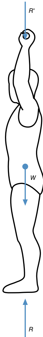
Figure 1.17 Free-body diagram of a weightlifter alone.
