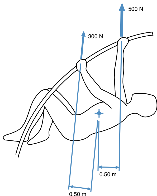
Figure 5.11 Free-body diagram of a pole-vaulter midway through the vault. The reaction forces from the pole create torques in opposite directions on the vaulter.
