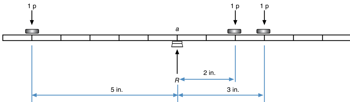
Figure 5.9 Free-body diagram of a ruler balanced on an eraser with pennies on the ruler. R is the reaction force exerted by the support of the ruler, and a is the axis. (The weight of the ruler is omitted in this diagram.)
