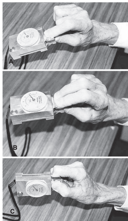
FIGURE 19.10 Use of a pinch meter to measure precision grip strength. Three types of pinch are examined: A, Tip-to-tip; B, Three-jaw chuck; C, Key or lateral grip.
