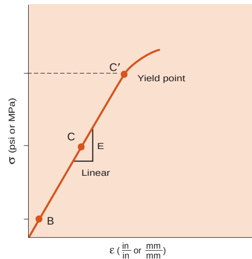
Figure 2.9: Yield. Another scenario for failure of the test specimens illustrated in Figures 2.4 and 2.5 is that the material's behavior is linear until point C'. At point C', the yield point, the stress-strain relationship is no longer linear, although the material does not break.
