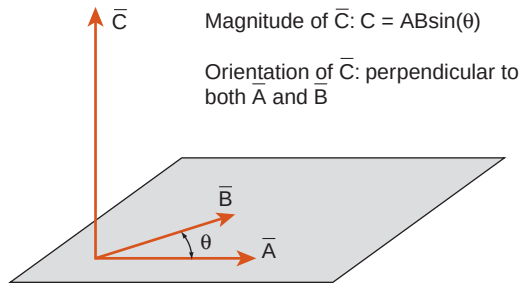
Figure 1.3: Vector cross product. \vec{C} is shown as the cross product of \vec{A} and \vec{B} . Note that \vec{A} and \vec{B} could be any two vectors in the indicated plane and \vec{C} would still have the same orientation.
