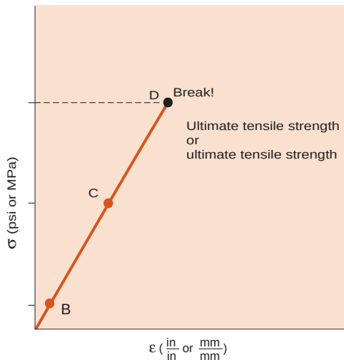
Figure 2.8: Brittle failure. One scenario for the failure of the test specimen illustrated in Figures 2.4 and 2.5 is that with a continued increase in load on the specimen, the specimen breaks at point D. Note that the stress-strain relationship remains linear. Point D represents the ultimate tensile strength of the material.
