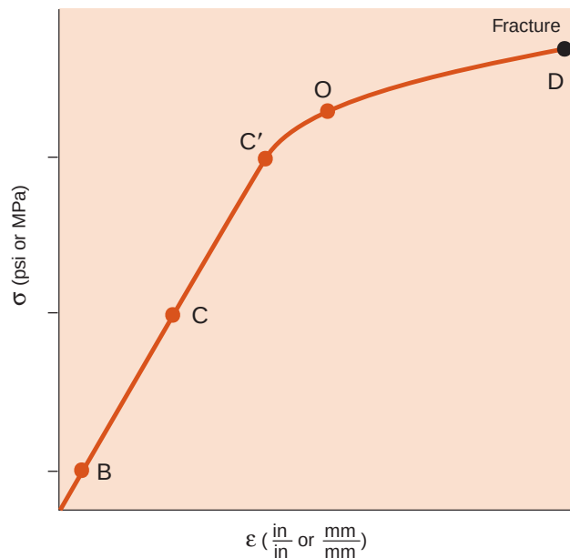
Figure 2.11: Ductile failure. After the specimen yields, with a continued increase in the applied load, the specimen eventually fractures (point D). Because the specimen yields before fracture, this is an example of a ductile fracture. For this ductile material, point D represents the ultimate tensile strength.
